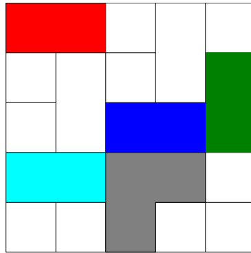
Figure 358: How the Randomized Kruskal's Algorithm Works (4/6)
